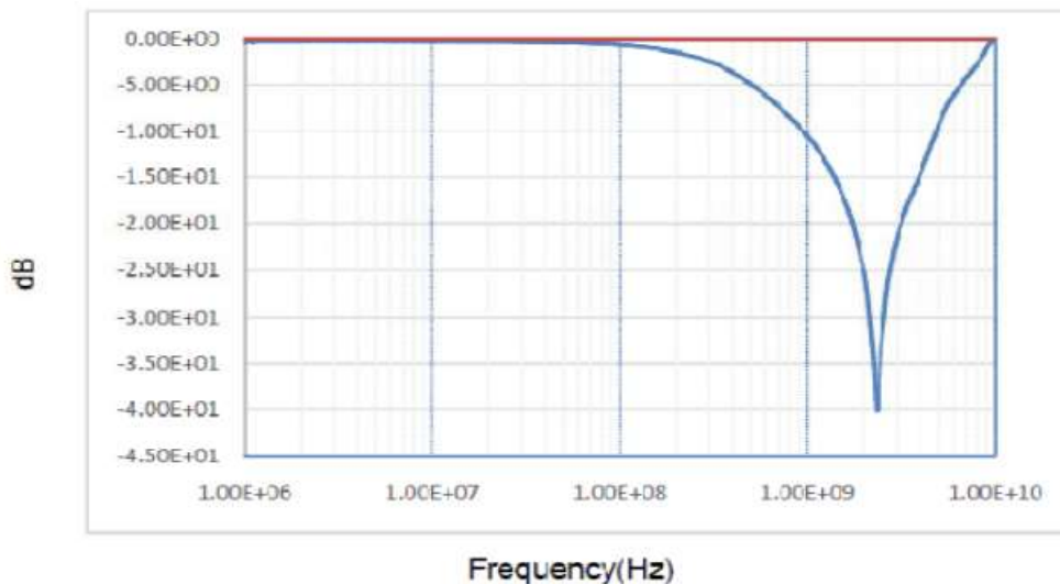
GBDC0605PT - 120N
