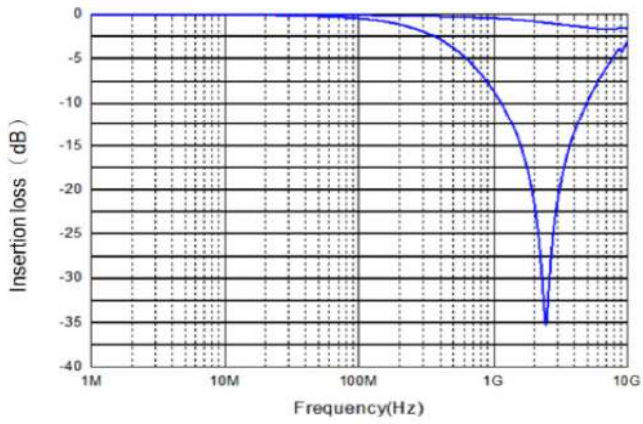
GBDC0806PS - 120N
