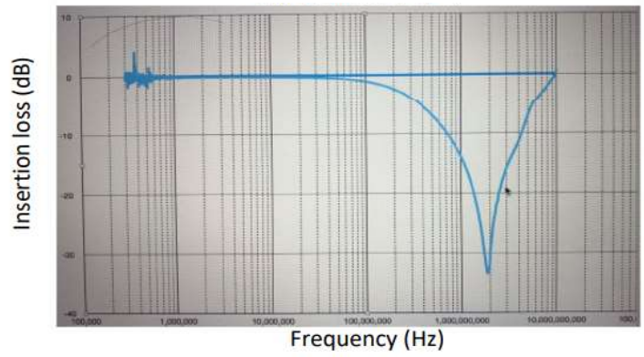
GBDC0806PS - 250N
