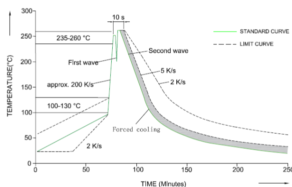
Temperature characteristic at component terminal with dual-wave soldering
